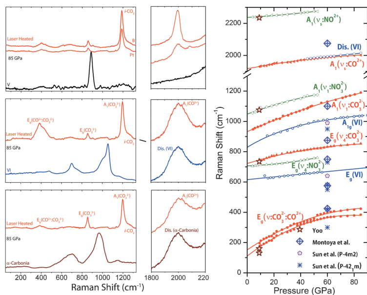
Figure 2. Left and center: Raman spectra of carbon dioxide phases before and after laser heating, showing the transformations of phase V (top), VI (middle), and amorphous \alpha -carbonia (bottom) to an extended form of ionic \text{CO}_2 carbonates ( i - \text{CO}_2 ), all at approximately 85 GPa and 1700–1800 K. Indirect Laser heating with Pt and B (top traces in each panel) had no effect on the reaction products, but the broad band at 2000 \text{cm}^{-1} appeared substantially sharper when using a boron heat absorber. Right: Pressure dependence of the Raman spectra of the ionic \text{CO}_2 phase (in red solid symbols and lines), plotted together with that of ionic \text{N}_2\text{O} (green open symbols and lines) for comparison. [18] Also shown are the Raman spectra of \text{CO}_3^{2-} previously synthesized by heating oxygen in carbon at 9 GPa (open stars) [17] and the calculated Raman spectra of the three-, four-, and mixedfold layered carbonates and m -chalcopryrite structures at 60 GPa (open symbols as labeled at the bottom). [20–22]
