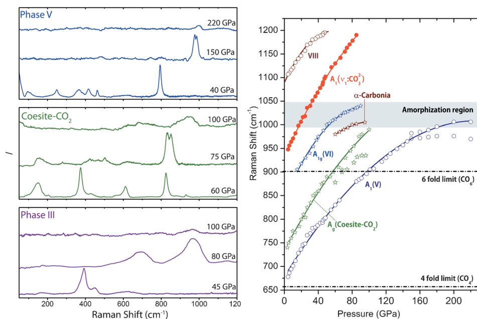
Figure 1. Left: Raman spectra of carbon dioxide phases to 220 GPa, showing the pressure-induced amorphization of top: fourfold \text{CO}_2 -V via a new high-pressure phase V' above 150 GPa, middle: coesite- \text{CO}_2 (c-I) via a high pressure-form (c-II), and bottom: phase III via \alpha -carbonia, at ambient temperature. Right: Pressure dependencies of the major \nu_6 vibrons of carbon dioxide phases, illustrating that pressure-induced amorphization occurs well beyond the sixfold vibron limit around 1000–1050 \text{cm}^{-1} (hatched area). The filled red colored circles are the symmetric stretching \nu_1 mode of carbonate ions (also in Figure 2).
